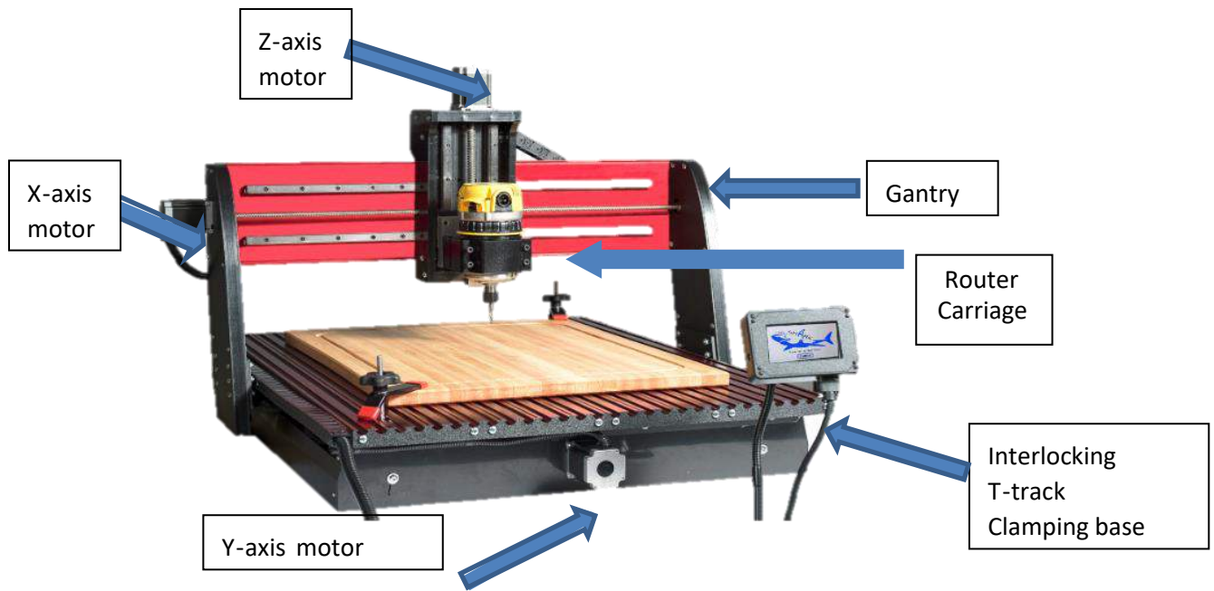
CNC Shark HD5 Core Components
